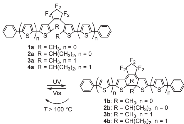
Scheme 1. Photochromic reactions of diarylethene derivatives.
