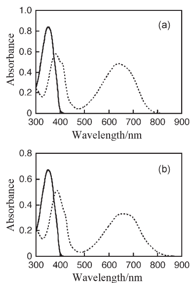
Figure 1. Absorption spectra of 3a (—) and 3b (----) (a) and 4a (—) and 4b (----) (b) in toluene at room temperature.
