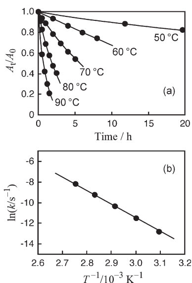
Figure 2. Decay curves (a) and temperature dependence (b) of thermal cycloreversion reactions of 4b in decalin.
