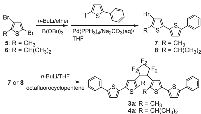
Scheme 2. Synthetic route of diarylethene derivatives.
